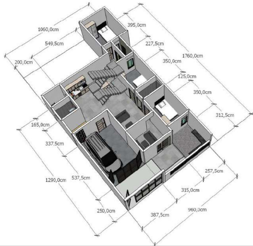
Denah Lantai 1 Ketinggian As Bangunan 3 Meter
